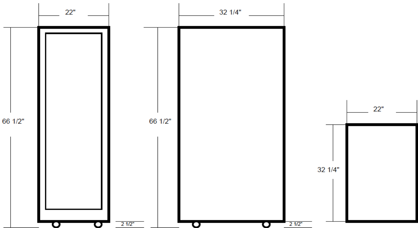
Front View
